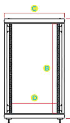
VISTA FRONTAL
